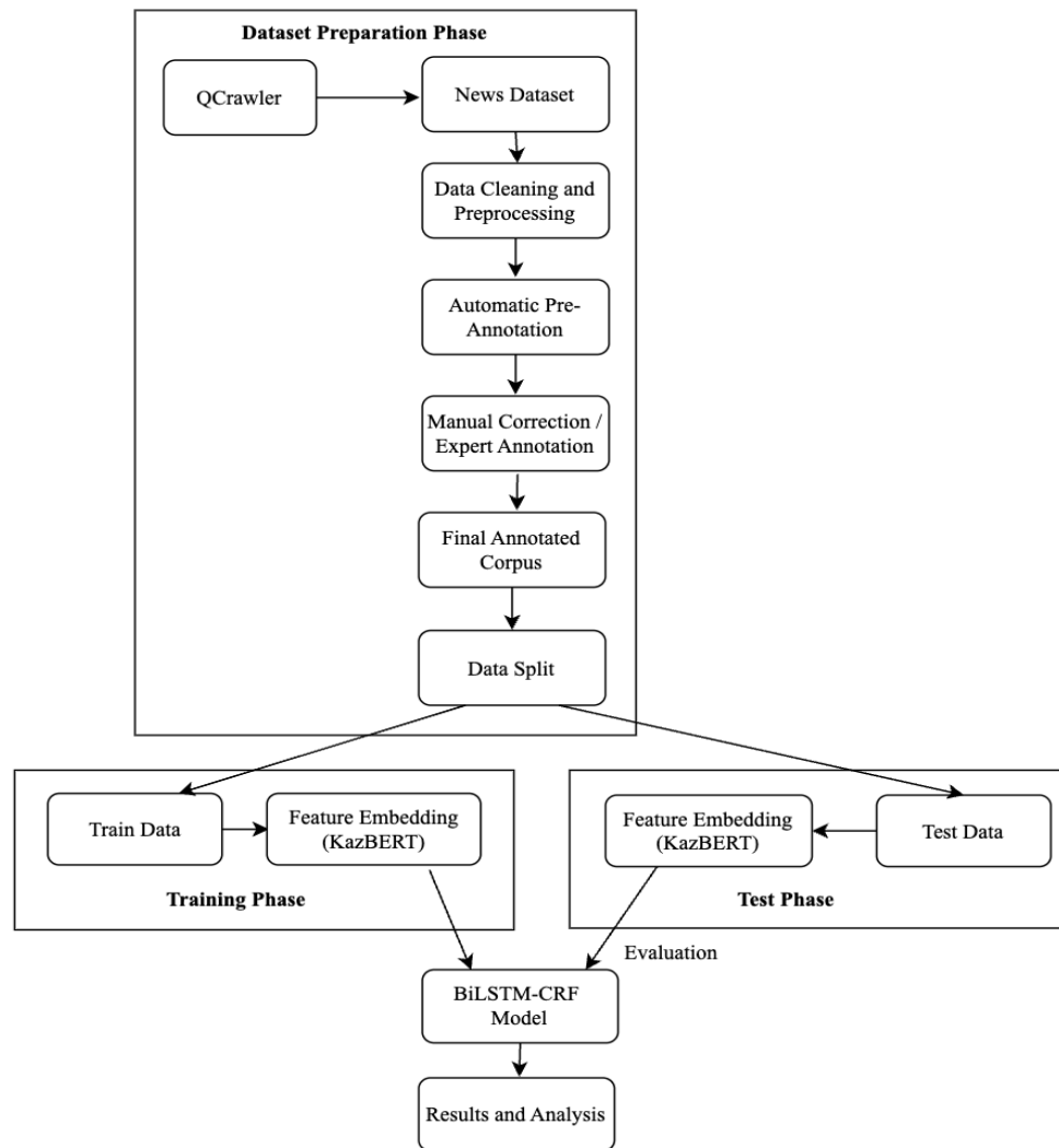
Figure 4.1 – End-to-end pipeline for Kazakh news corpus construction and model training
