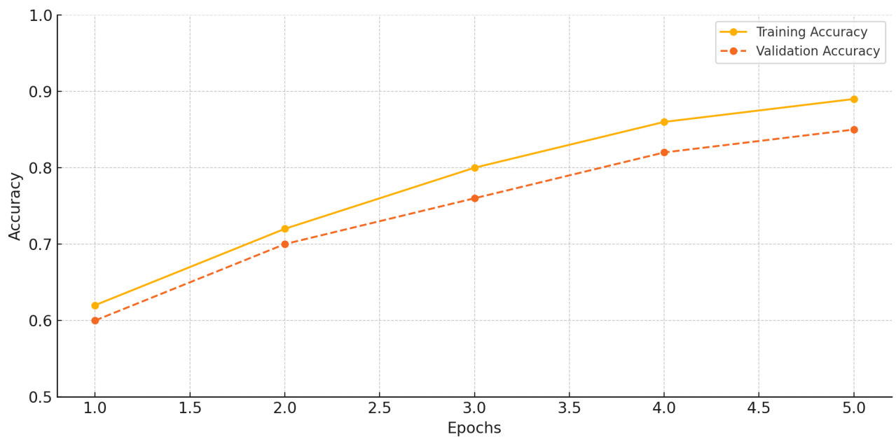
Figure 4.10.2 - Training vs validation accuracy progression over epochs in QNLP
