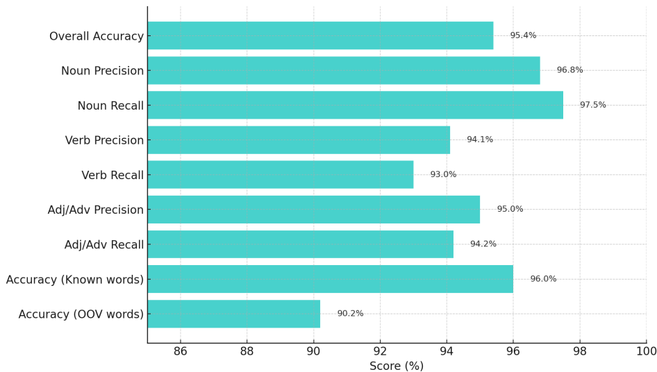
Figure 4.7.1 - POS Tagging results on Kazakh test set
