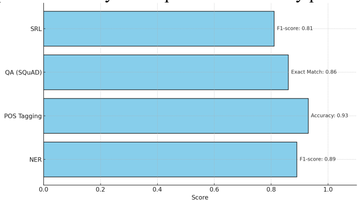
Figure 4.7 - Evaluation Metrics
